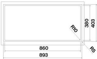
Cut-out size for flushmounted installation
