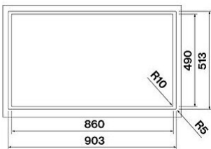
Cut-out size for flushmounted installation
