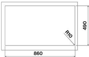
Cut-out size for topmounted installation
