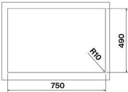
Cut-out size for topmounted installation
