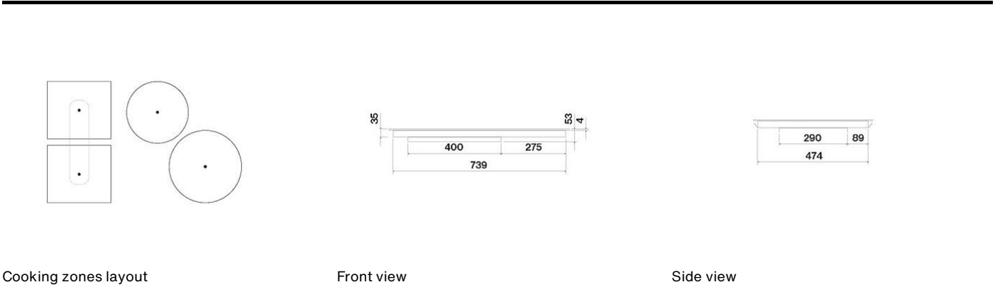
Cooking zones layout
