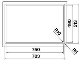
Cut-out size for flushmounted installation
