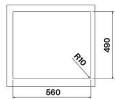
Cut-out size for topmounted installation
