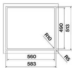
Cut-out size for flushmounted installation
